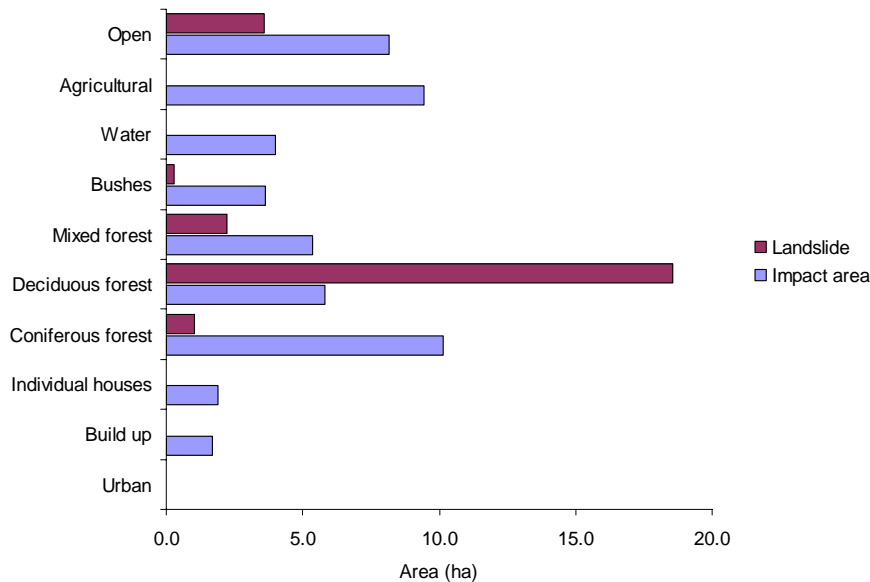
Figure 5. Land use classes destroyed by the landslide.
