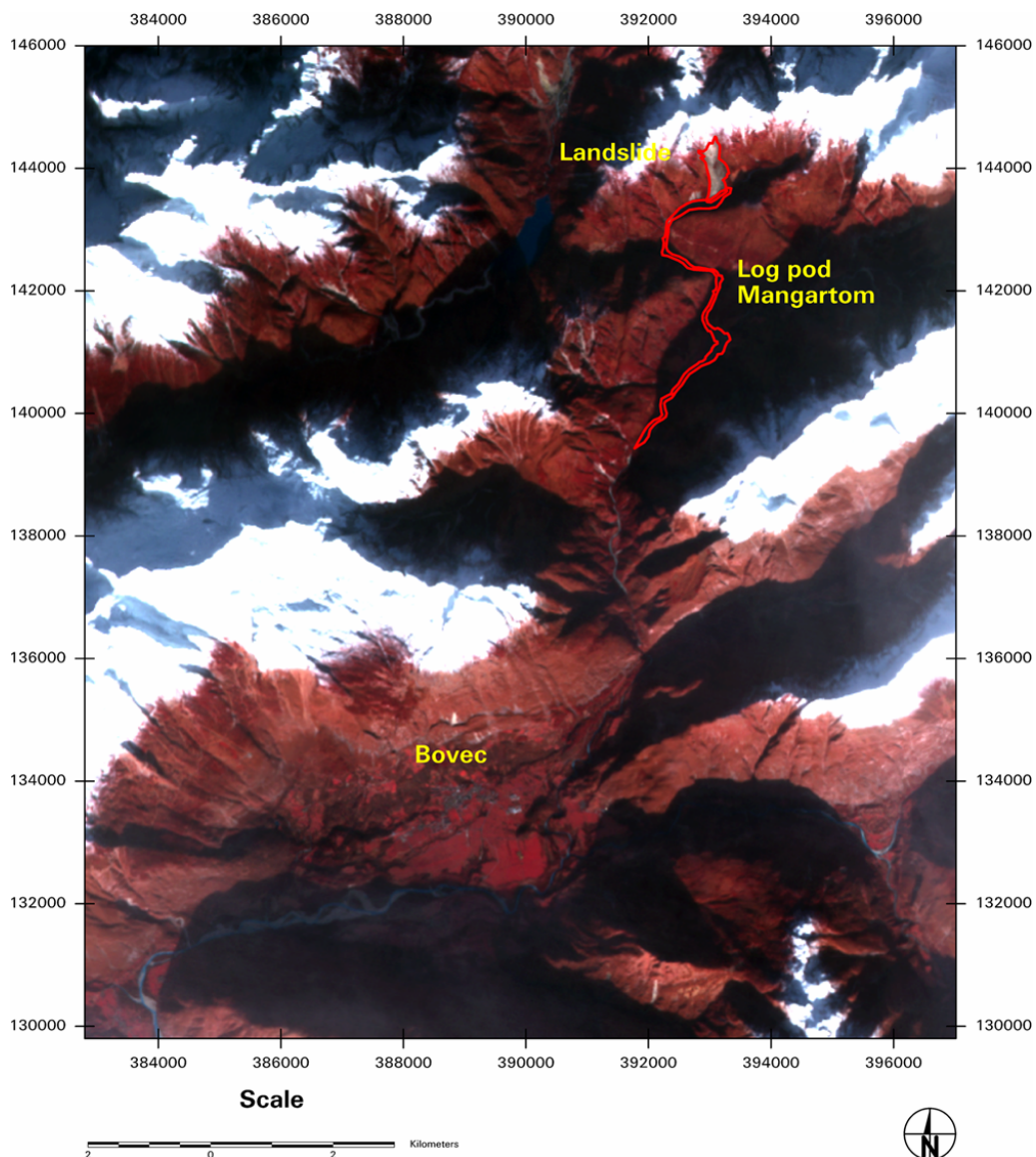
Figure 4. SPOT satellite map of landslide area (image was acquired on 29 November 2000).
