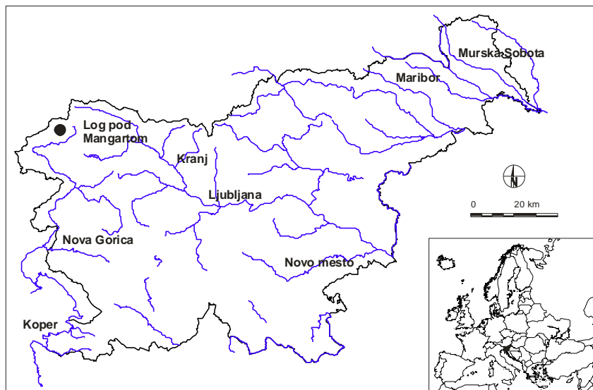
Figure 3. Location of the Mount Mangart landslide.
