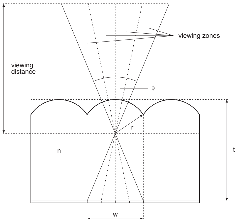
Figure 2: Parameters of the lenticular foil.
