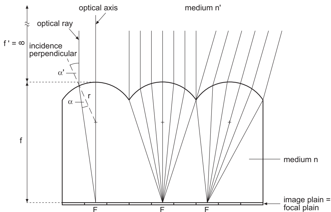
Figure 3: Optical paths in the lenses.
