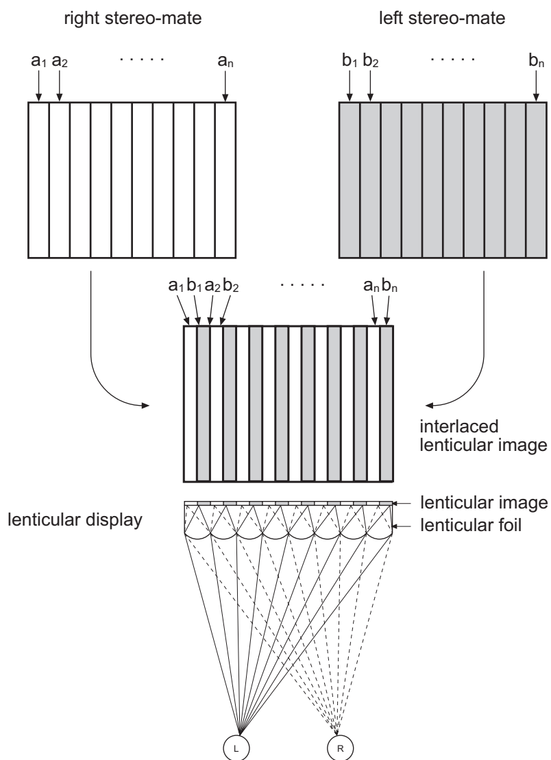
Figure 1: Interlacing of "subimages" and principle of 3D-lenticular method.
