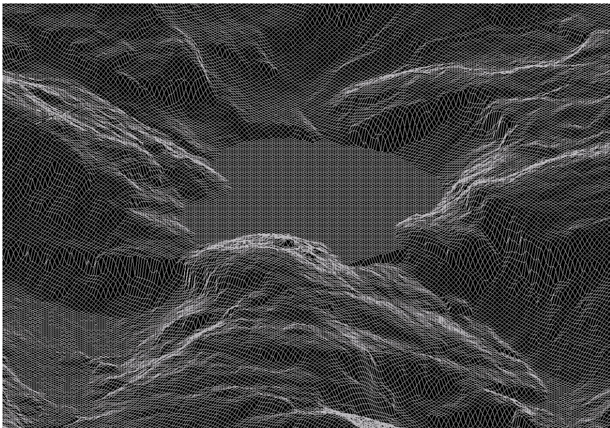
Figure 5: Grid DTM, view of Weisssee from north-east. For the visualisation grid-width decreased to 10 m.
